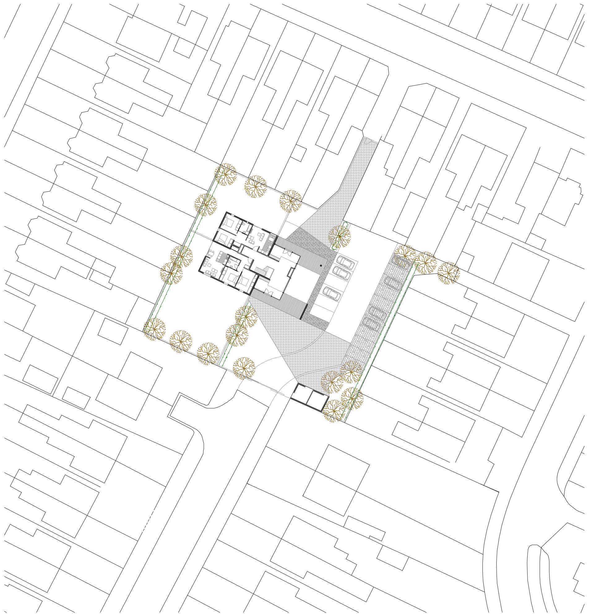
Proposed site plan Southport 1 5 10 15 meter
